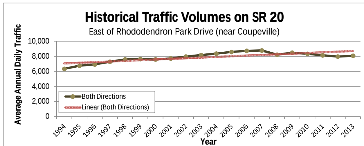
Exhibit 2-1 Historical AADT for SR 20
